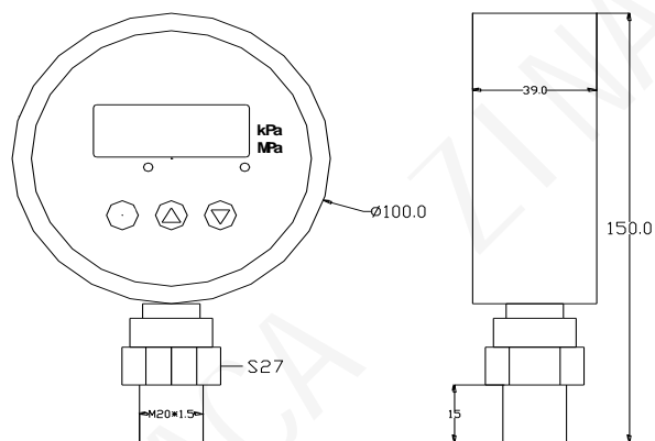
Standard pressure controller (protection class IP54)
