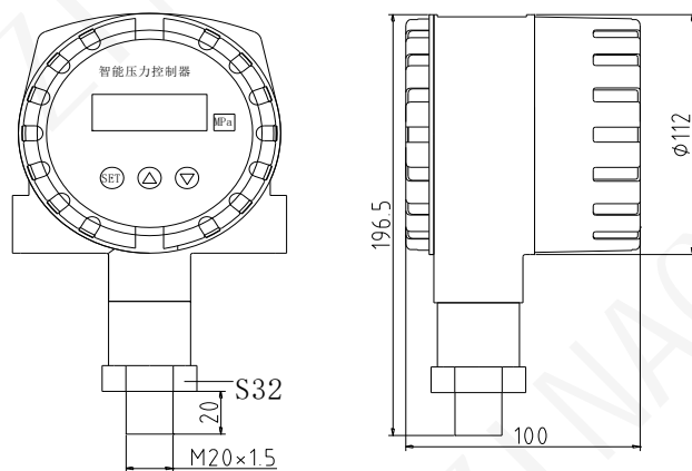
Explosion-proof pressure controller (protection class IP65)
