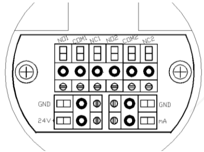
D. Intelligent pressure controller (two switching with one 4-20mA output)
