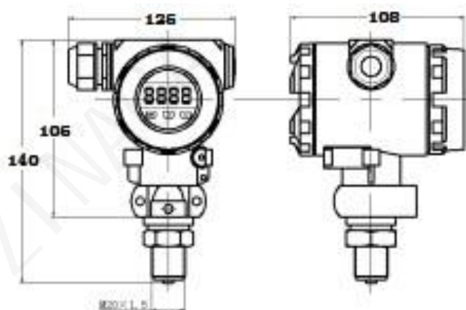
Intelligent pressure controller (protection class IP65)
